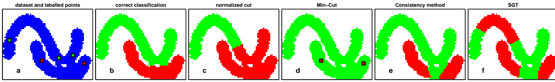
Figure 1. a. The unlabelled data in blue; labelled points are marked in green and in red. Each of the 1360 pixels correspond to a data point; the labeled pixels were enlarged for clarity. b. The correct classification. c. Clustering results of the unsupervised normalized cut algorithm (Shi & Malik, 2000). d. The min-cut solution. e. The results of the semi-supervised consistency method of (Zhou et al., 2003). f. The outcome of the spectral graph transducer algorithm (Joachims, 2003), which is a semi-supervised extension of the normalized cut algorithm.
